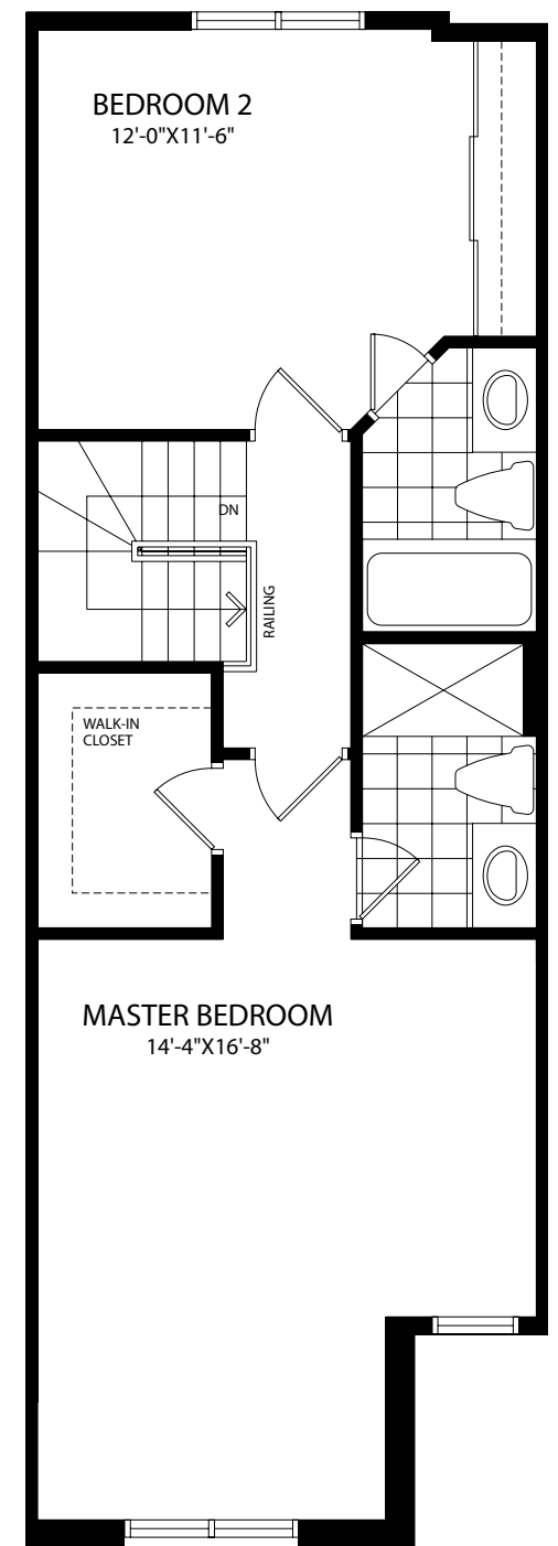
OPTIONAL UPPER FLOOR 2 BEDROOM
