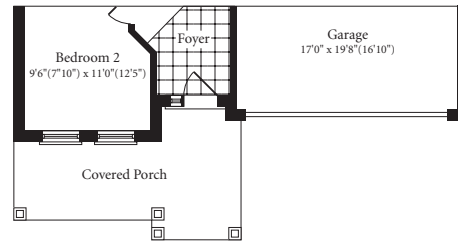
MAIN FLOOR, Elevation B
